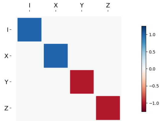
Figure 2: PTM of Pauli X gate
