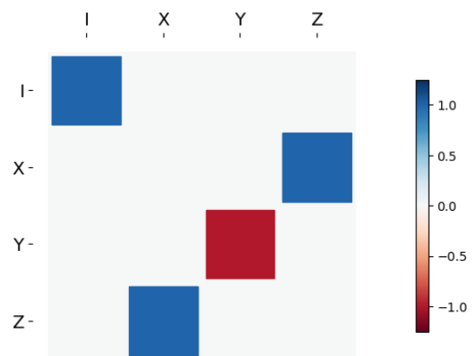
Figure 6: PTM of Hadamard gate
