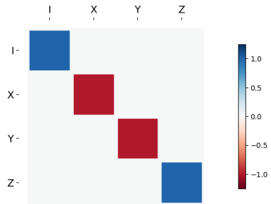
Figure 4: PTM of Pauli Z gate
