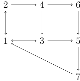
Figure 8: Diagram of the implications to prove the equivalence of Theorem 4.2
